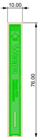
Front view
