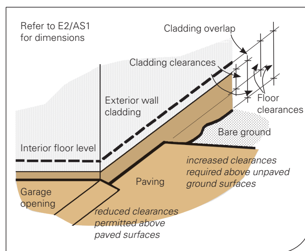
Figure 32: Adequate clearances
