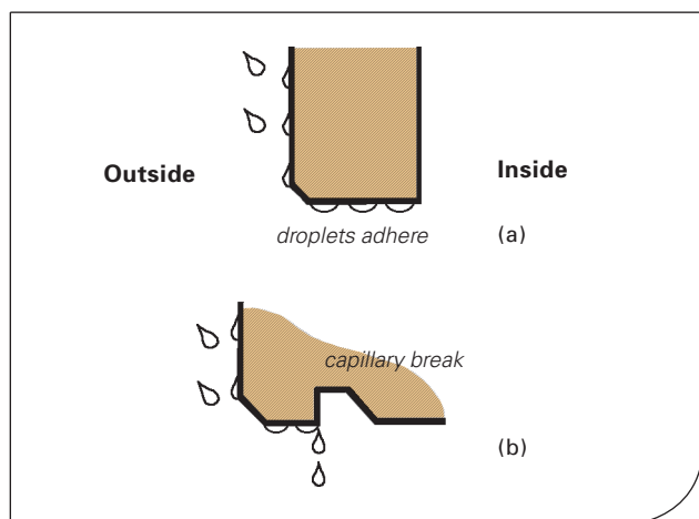
Figure 7: Water droplets
