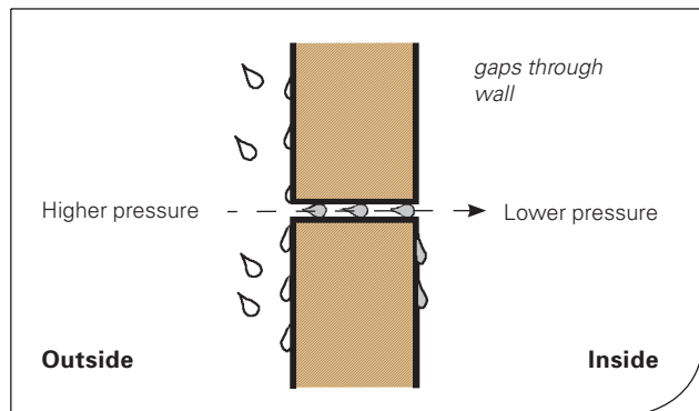
Figure 6: Pressure differentials
