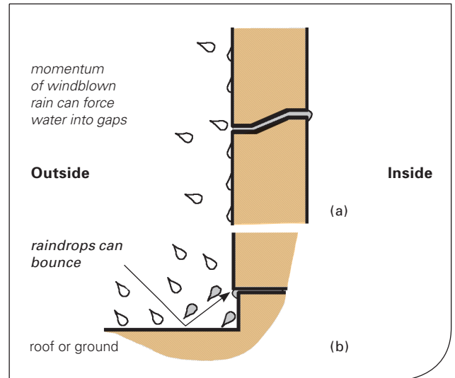
Figure 5: Momentum leaks
