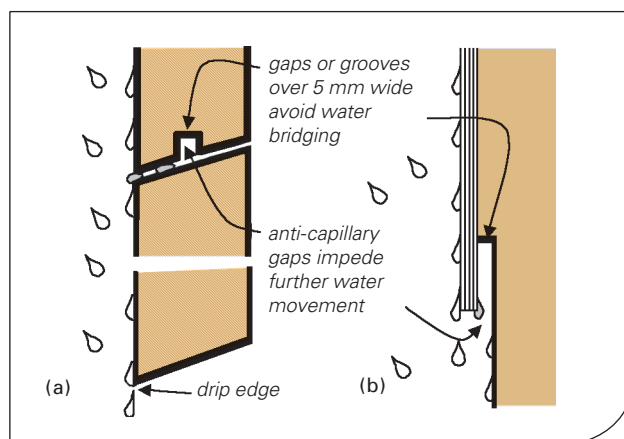
Figure 25: Anti-capillary separation
