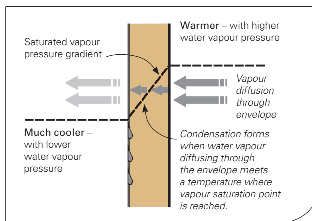
Figure 10: Interstitial Condensation
