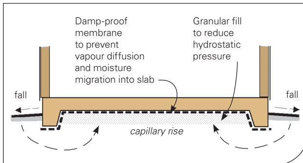
Figure 35: Concrete slab-on-ground
