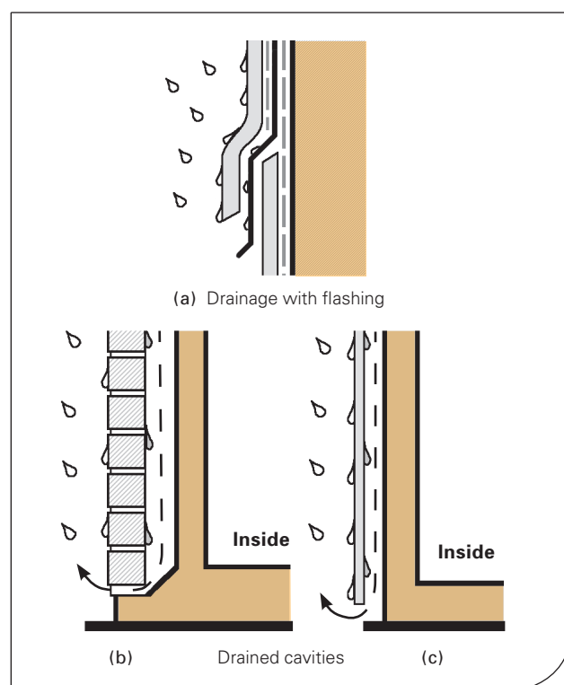
Figure 16: Drainage
