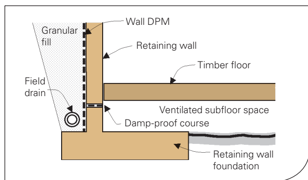
Figure 38: Retaining wall with raised floor
