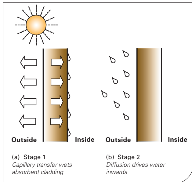
Figure 11: Solar-driven moisture
