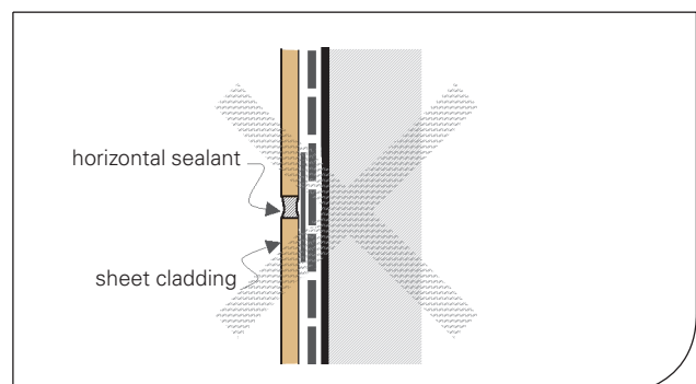
Figure 28: Sealant joints
