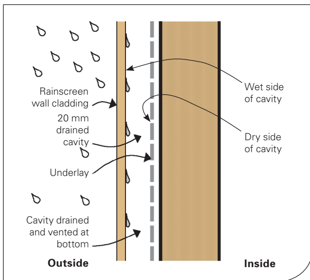
Figure 21: E2/AS1 drained cavity
