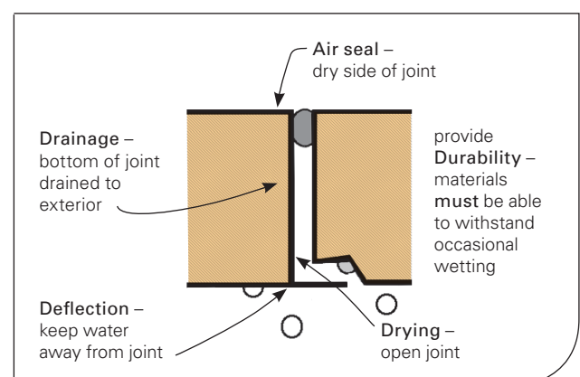
Figure 23: Vertical joint
