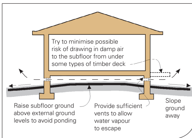
Figure 34: Timber-framed floors
