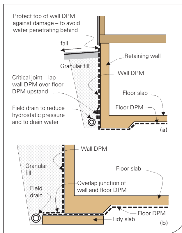
Figure 36: Wall/slab
